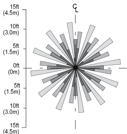
Low Bay Lens (N) Pattern
