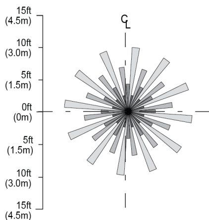
High Bay Lens (H) Pattern
